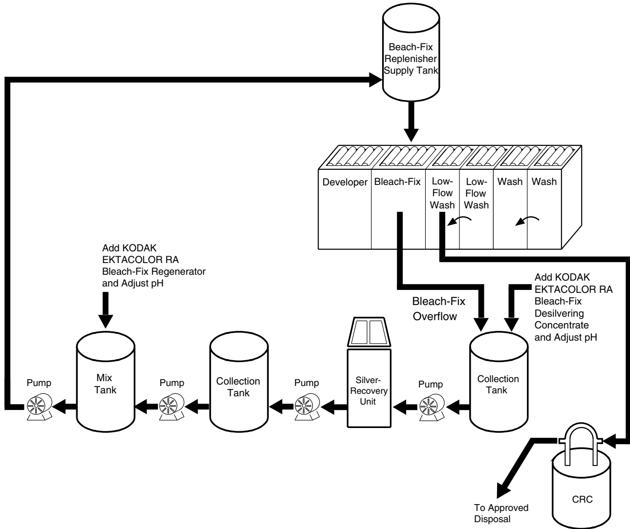
Figure 1 Regenerated Bleach-Fix System
